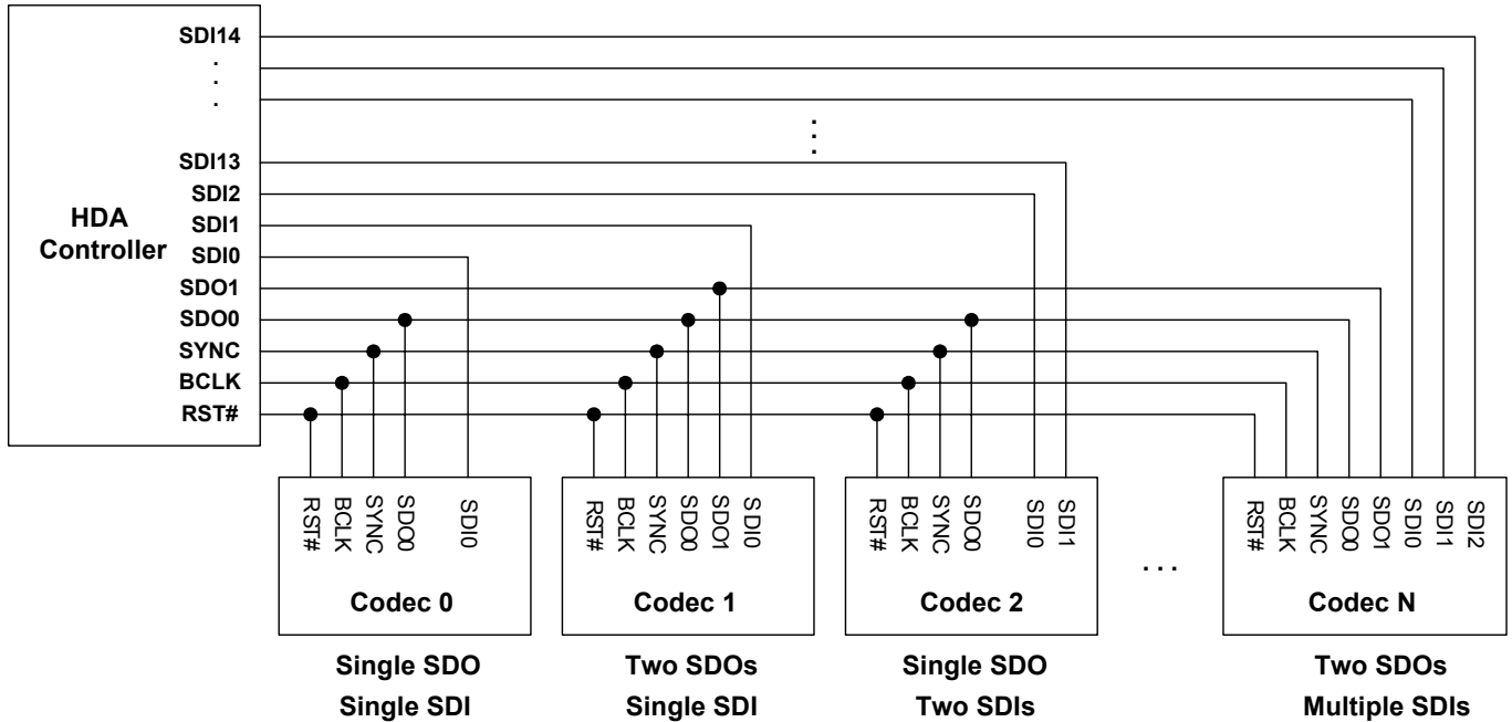
Figure 6. Signaling Topology
