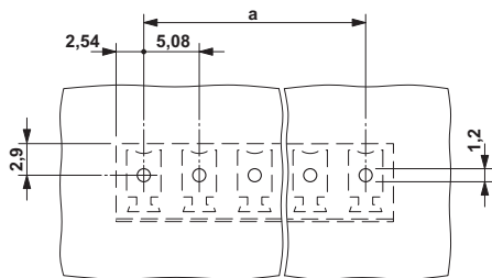
Drilling diagram
