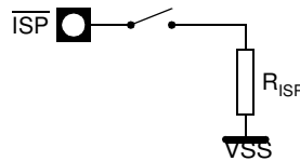
Figure 22-8. ISP Pull-Down Connection
