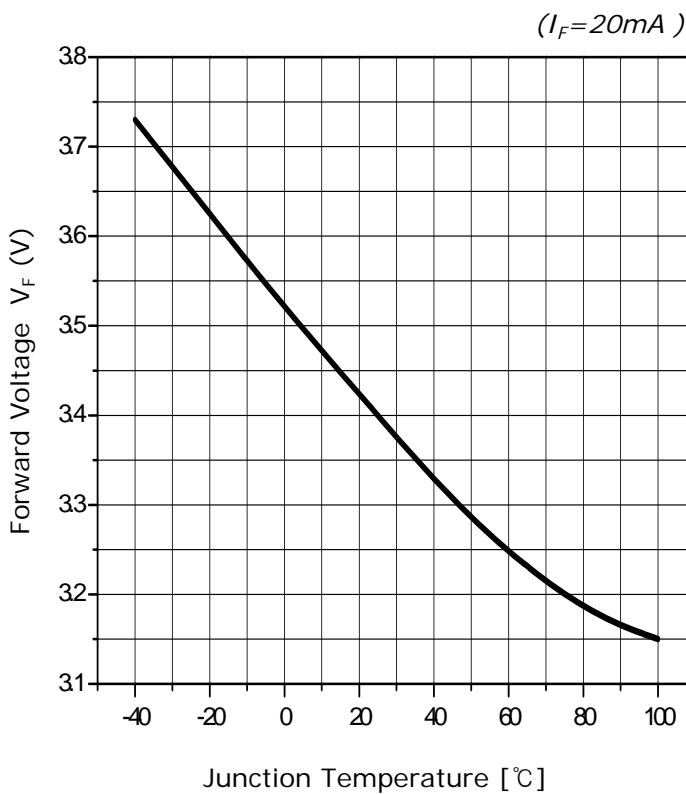
Forward Voltage vs. Junction Temperature
