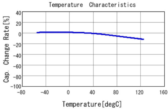
■ KRM55WR71E476MH01 C-Temp. capchange, DCOV, ACO, 5Vrms
