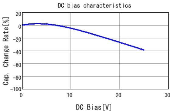
■ KRM55WR71E476MH01 C-DC bias capchange, 25.0degC, AC0.
