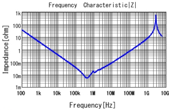
■ KRM55WR71E476MH01 |Z| DCOV, 25degC
