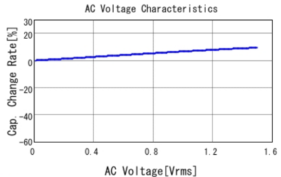
■ KRM55WR71E476MH01 C-AC Voltage capchange, DCOV, 25.0d
