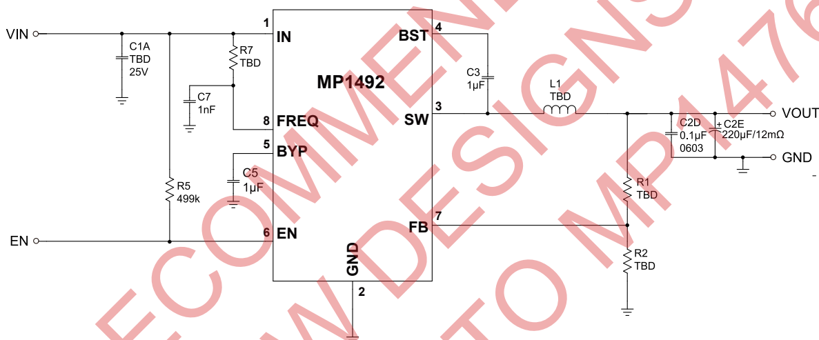
Figure 11—Typical Application Schematic with No External Ramp
