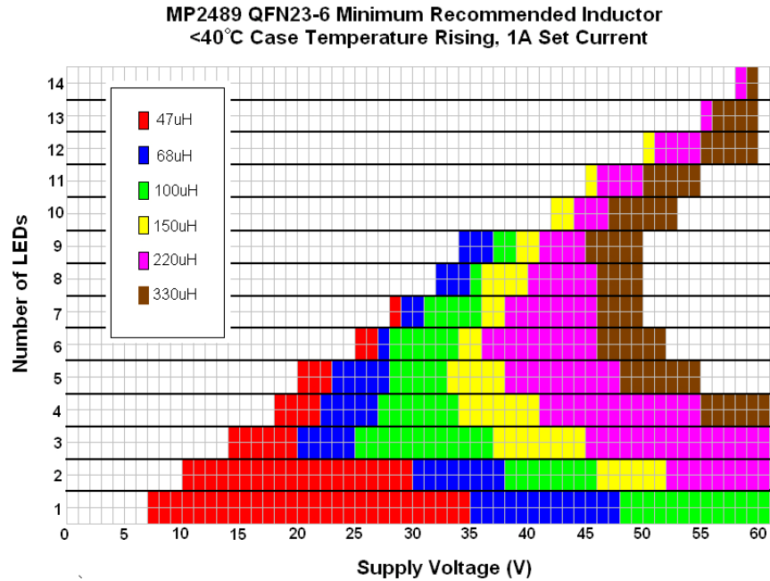
Figure 4—Inductor selection instruction for QFN23-6
