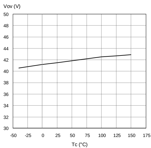
Figure 25. Overvoltage Shutdown
