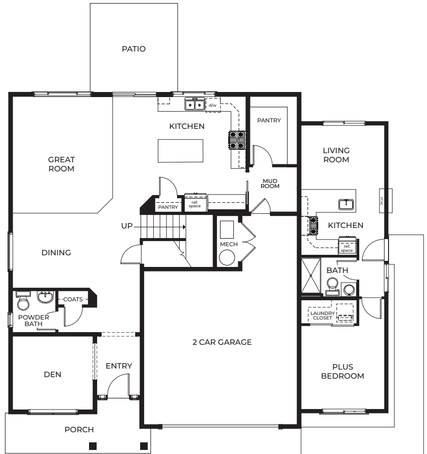
Main Floor
