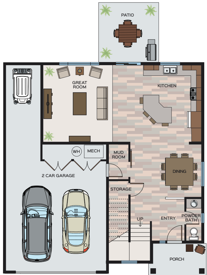
MAIN FLOOR
