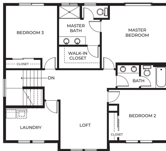
Upper Floor
