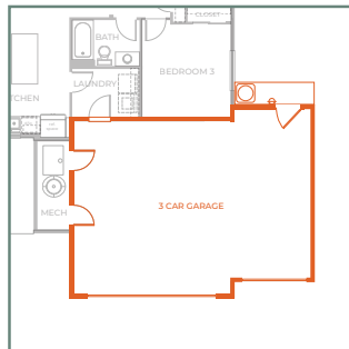
3 Car Contemporary Garage
