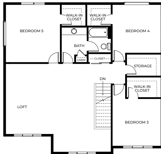
Upper Floor
