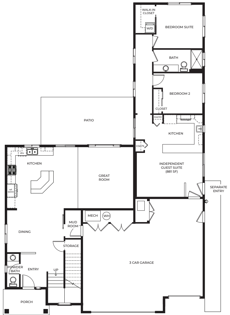
Main Floor
