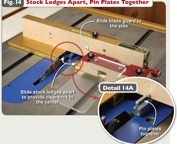
Fig. 14 Stock Ledges Apart, Pin Plates Together
