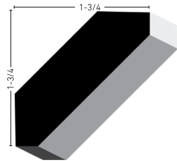
200 11/16 x 2-1/2 MDF 16'
