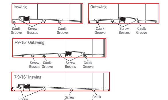
Template for 4-9/16" up to 7" inswing/outswing sills and 7-9/16" outswing sills
