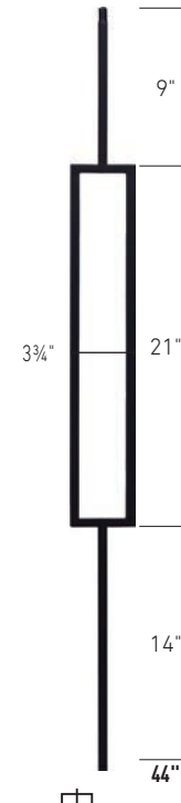
301 | 1/2" Single Rectangle
