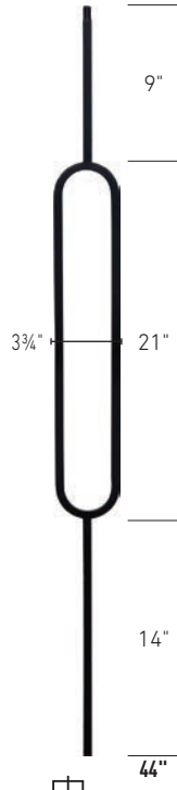
300 | 1/2" Oval Craftsman
