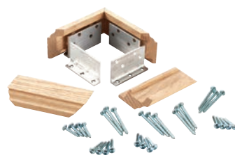
3009 - 3" Angle Bracket Post Fastener Kit 3019 - 3-1/2" Angle Bracket Post Fastener Kit ANGLE BRACKET POST FASTENER 3019MD - Trim Moulding Only
