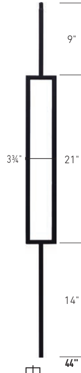
1663 44 1/2" Contempo Rectangle
