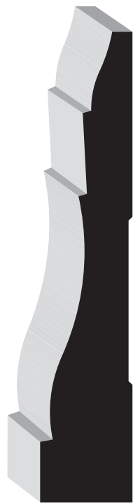
OE361 LWM361 11/16" x 3-1/2" SP RL
