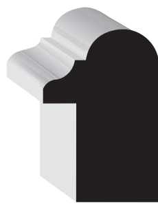
CR003 7/8" x 1-5/16"
