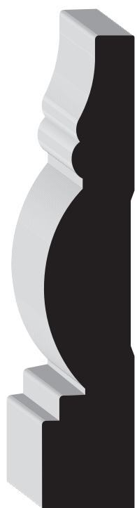
94112 3/4" x 3-1/2" PMDF 16'
