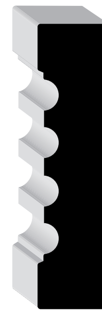
08583 3/4" x 3" PMDF 8'
