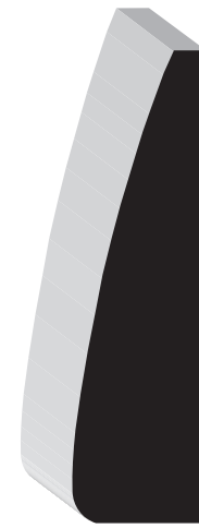
OW316 WM316 11/16" x 2-1/4" PFJP • SP 8', 16' • 7', RL
