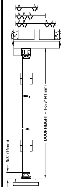
1725AOSB Components
