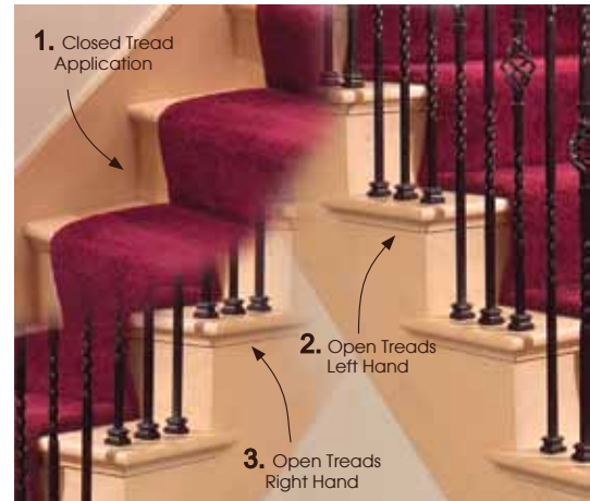
LJ-8879 Double Miter Return False Tread Kit This kit can accommodate applications 1, 2 or 3, as pictured above. Tread with attached moulding is 12 5/8" x 7 5/16" (321 mm x 186 mm) Riser is 7 3/4" x 6 1/2" x 1/2" (197 mm x 165 mm x 13 mm)
