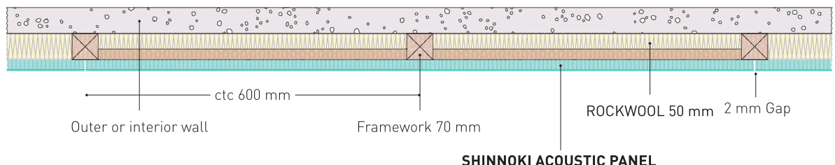
TOTAL THICKNESS WALL 87 mm
