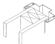
SLIP-ON DRYWALL (Interior Application)
