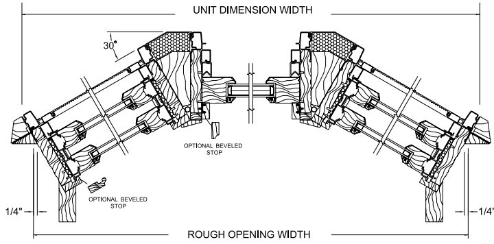
30° Bay Horizontal Section
