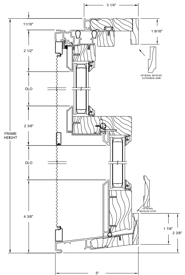
Vertical Section
