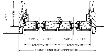
Horizontal Section
