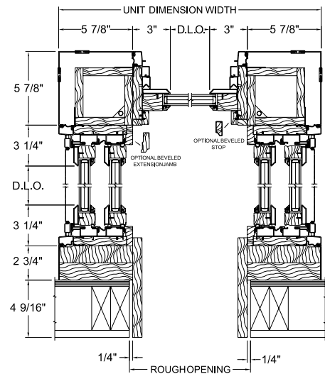
90° Bay Horizontal Section
