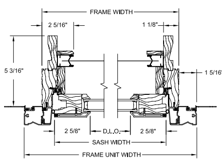
Horizontal Section – multi-point lock
