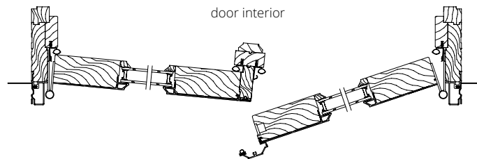
AL (French, Hinged Right, Active)
