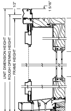
Vertical Section
