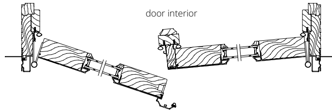
AR (French, Hinged Left, Active)
