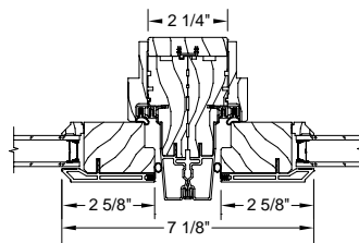
Narrow Mullion
