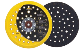
916GV 6" Backup Pad Medium, Multi-Hole, Grip 5/16" - 24 thread
