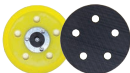
105GV 5" Backup Pad Medium, 5-Hole Grip, 5/16 - 24 thread
