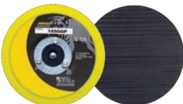
105GGP 5" Backup Pad Medium, Grip, J Hook 5/16 x 24 thread
