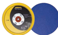
105H 5" Backup Pad Medium, PSA, Hardened Shank, 5/16 - 24 thread
