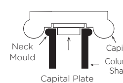
8"-12" Load Bearing Capital
