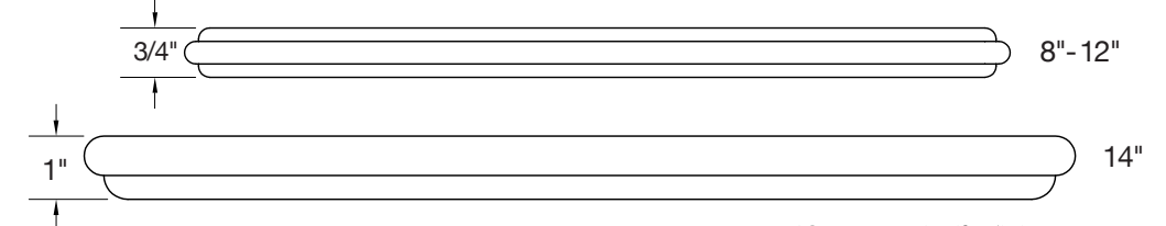
Neck Mould for No-Taper Column - Sold Separately.
