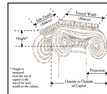
14"- 30" Non Load Bearing Capital with Separate Load bearing Plug
