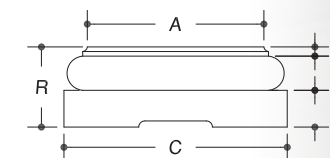
Standard Poly Base
