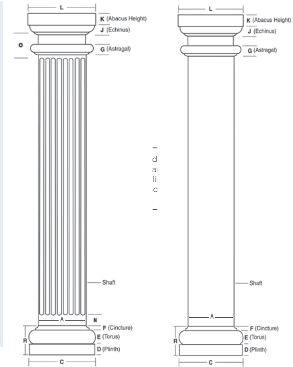
PermaCast® Plus Square Column shown fluted with Poly Tuscan Cap and Base.
