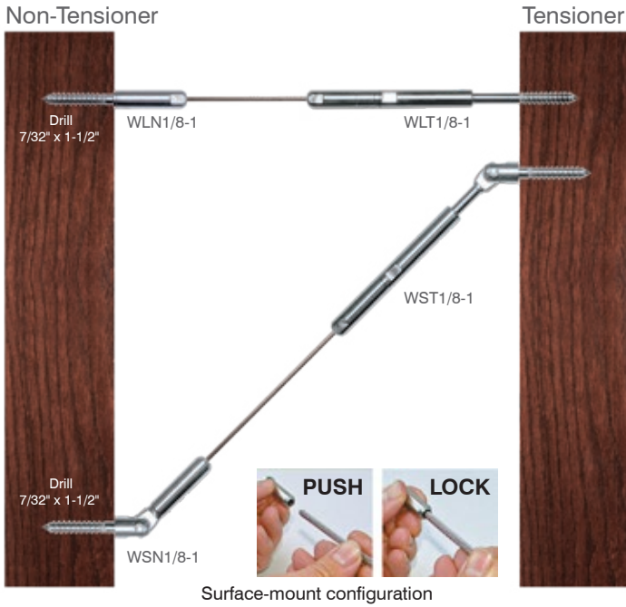
Surface-mount configuration
