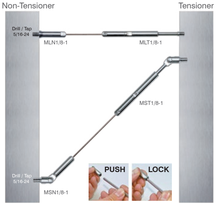
Surface-mount configuration
