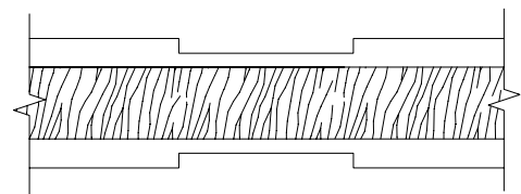
Groove Detail 9/16" wide x 1/16" deep
