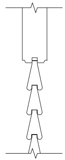
OPTIONAL CHEVRON NON-VENTED LOUVER Available in 1-3/4" only
