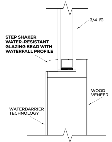
OPTIONAL SHAKER PROFILE WITH WATERBARRIER® TECHNOLOGY
