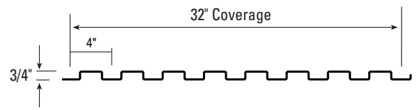
T16-E Wall
