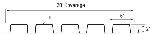
T2630 Wall
