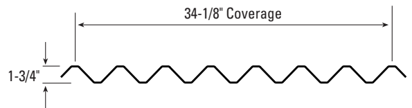
T16-L Wall
