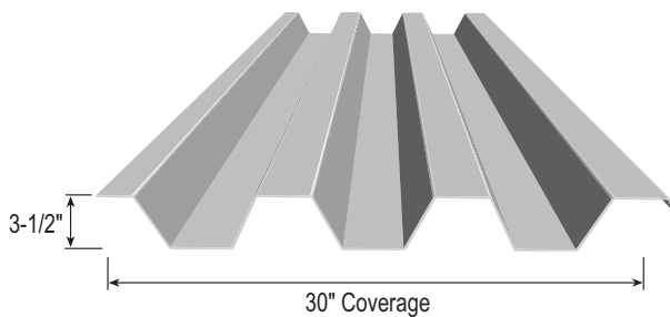
T14 Roof
