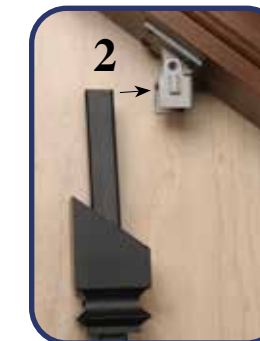
Slide Iron Baluster In Place With Shoes Installed
