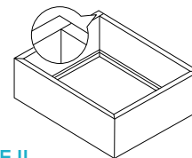
TYPE II Four sided drawer 3 mitered corners, 1 butt joint
