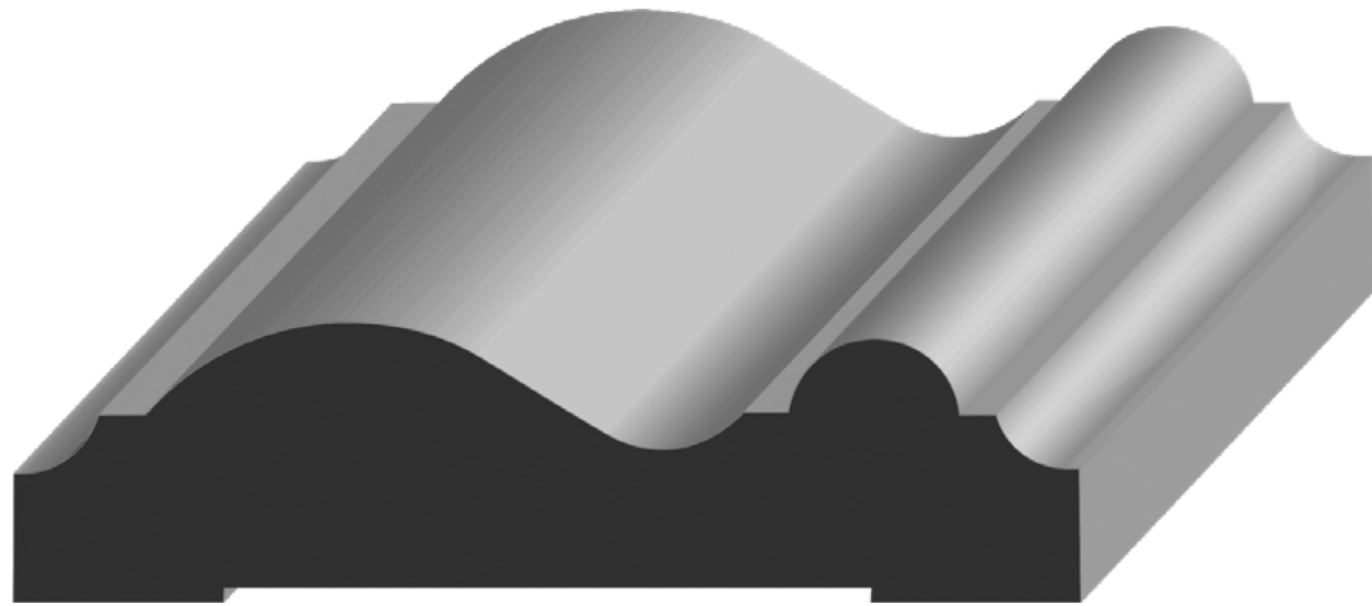
PX 431 1-3/8" x 5-3/16"
