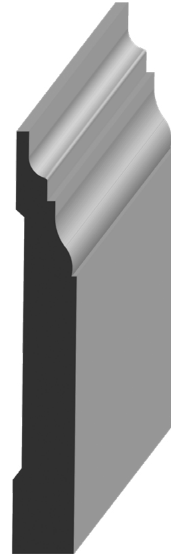
PX 662 25/32" x 5-1/2"
