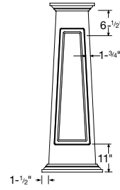
Route is 1-3/8" wide by 3/8" deep.
