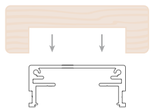
SERIES 450 Low Profile for Optional Cap (not included)
