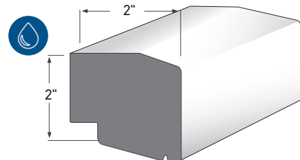
LARGE SILL NOSE AZM-7979 LENGTH: 16'
