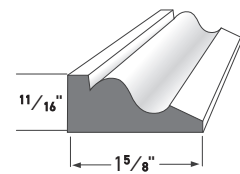
BAND MOULDING AZM-217 LENGTH: 16'
