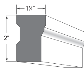
BRICK MOULD AZM-180 LENGTHS: 16', 17' and 18*
