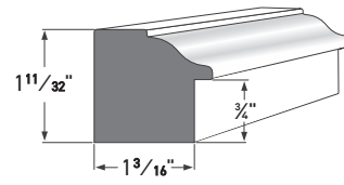
BACK BAND AZM-6931 LENGTH: 16'
