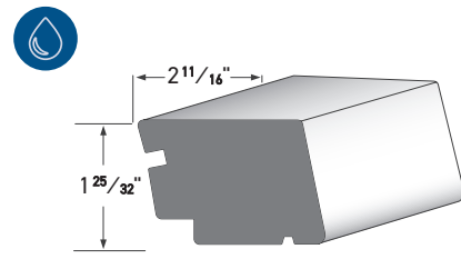
LARGE HISTORIC SILL AZM-7958 LENGTH: 16'
