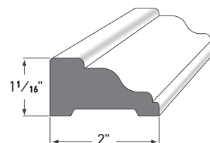
RAKE MOULDING AZM-287 LENGTH: 16'
