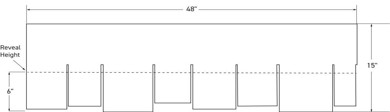
6" REVEAL STAGGERED-EDGE SHINGLE PANEL (50 panels per square)
