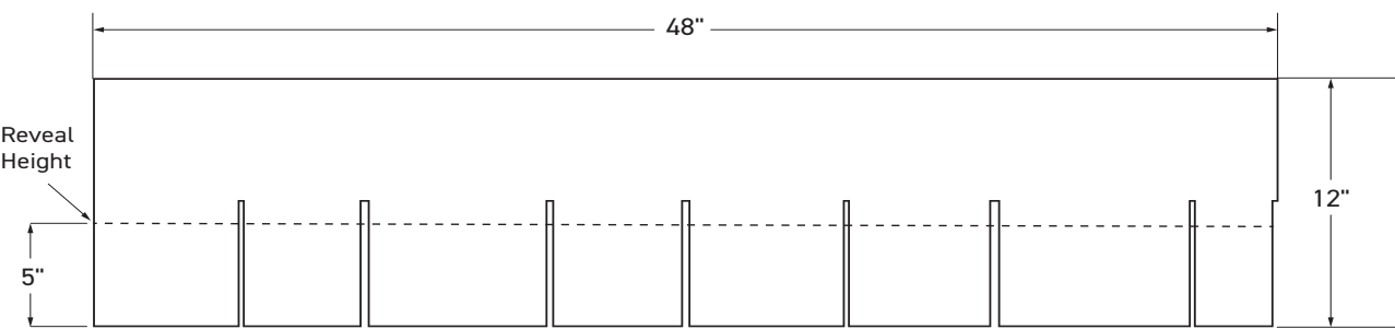
5" REVEAL STRAIGHT-EDGE SHINGLE PANEL (60 panels per square)
