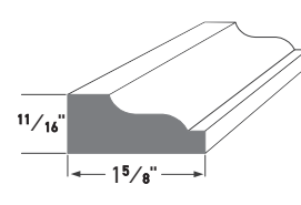
SHINGLE MOULD AZM-210 LENGTH: 16'
