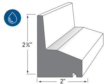
WATER TABLE AZM-6935 LENGTH: 18'
