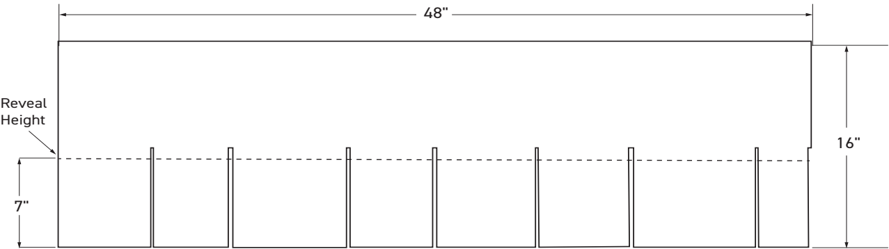
7" REVEAL STRAIGHT-EDGE SHINGLE PANEL (43 panels per square)
