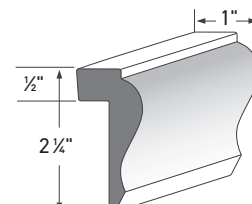
WAINSCOT CAP AZM-284 LENGTH: 16'
