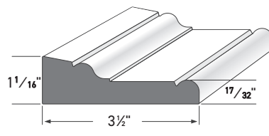
ADAMS CASING AZM-97 LENGTH: 16'
