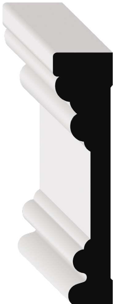
STOCK CODE 34136CAPRI (1521783) DIMENSIONS 1 1/16" x 4 1/4" x 17' PRI
