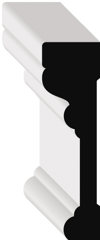
STOCK CODE 34112HCAPRI (1521781) DIMENSIONS 1 1/16" x 3 1/2" x 15' PRI
