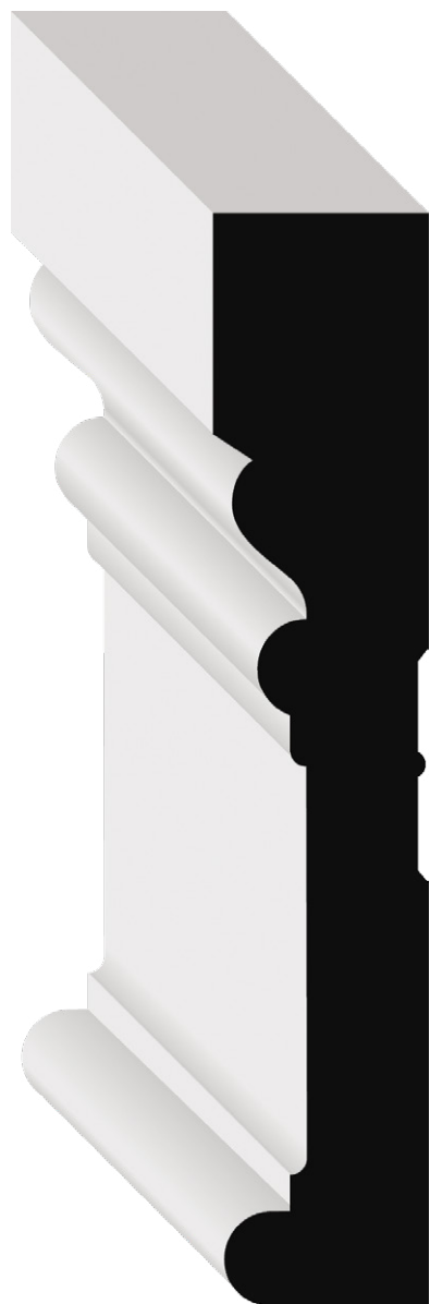
STOCK CODE 190DHM (1521466) DIMENSIONS 1\frac{1}{16}" \times 5\frac{5}{16}" \times 16' MDF/UL
