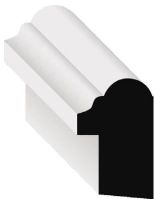
STOCK CODE 2844BBP (1521718) DIMENSIONS \frac{7}{8}" \times 1\frac{3}{8}" \times 16' FITS 1\frac{1}{16}" TO \frac{3}{4}" CASING PFJ
