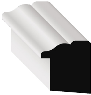
STOCK CODE 3436BBPOP (1521789) DIMENSIONS 1\frac{1}{8}" \times 1\frac{1}{16}" \times 6-16' FITS 1\frac{1}{16}" TO \frac{3}{4}" CASING POP
