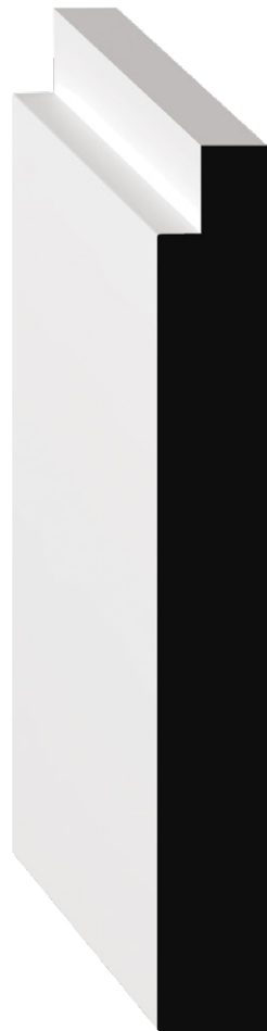
STOCK CODE 1680072 DIMENSIONS \frac{5}{8} " x 4\frac{1}{4} " x 16' MDF/UL
