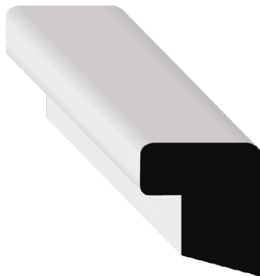
STOCK CODE 9701PRI (1522368) DIMENSIONS \frac{3}{4}" \times 1\frac{3}{16}" \times 16' FITS \frac{1}{2}" CASING PRI
