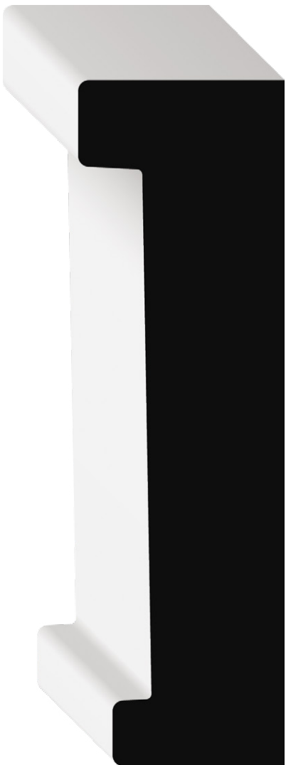
STOCK CODE CTC1A1PMD12 (1322025) DIMENSIONS 1 1/2" x 5" x 12' MDF/UL
