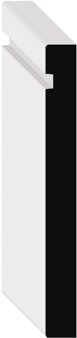
STOCK CODE 9290MDF (1626240) 9291M (1626242) DIMENSIONS \frac{1}{2}" \times 5" \times 16' \frac{1}{2}" \times 6\frac{1}{2}" \times 16' MDF/UL
