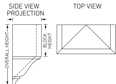
MIDDLE BLOCK
