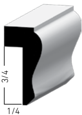
PLY CAP
