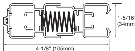
Screen Panel Profiles with Pleated Fabric
