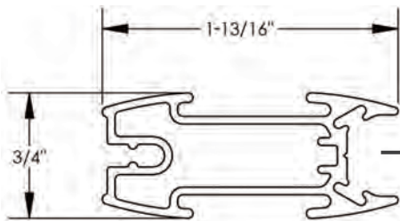
Slider Bar Profile
