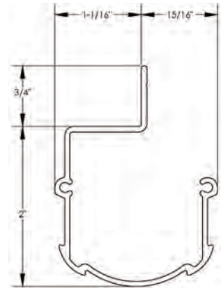
Screen Housing Profile
