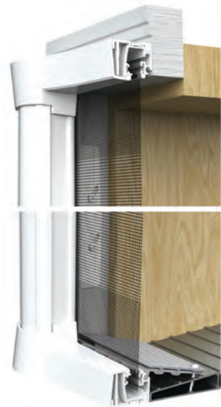
Surface / Face Mounting on a Traditional Hinged Door.
