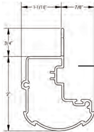
Decorative Housing Profile
