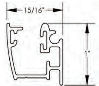
Top Track / Bottom Track
