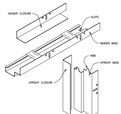
REDIFLEX CORNER DETAIL
