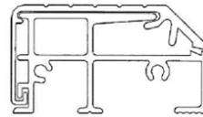
Fixed Vinyl Riser (Included in Fixed Sill Base Kit)
