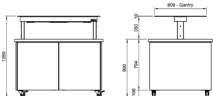
Front Elevation
