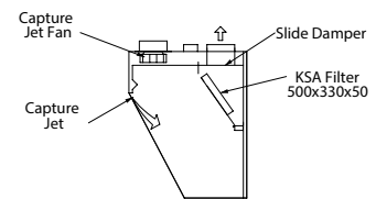
Typical End View
