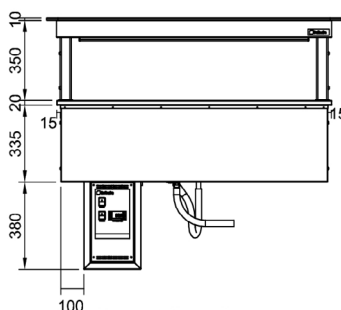
Front Elevation
