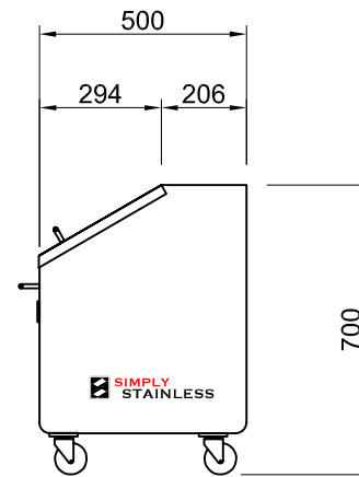
SIDE ELEVATION
