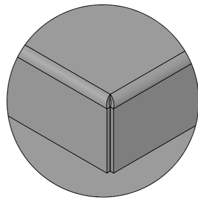
DETAIL K
