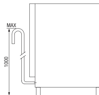
DRAIN HEIGHT
