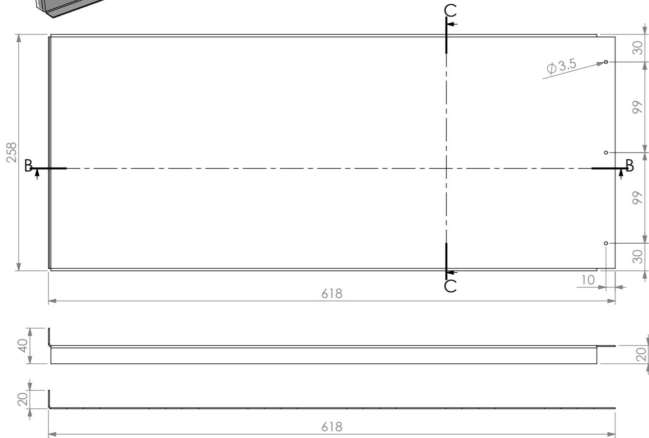
SECTION B-B
