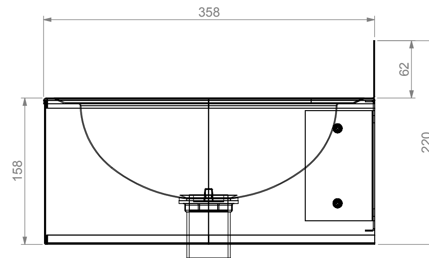
END VIEW
