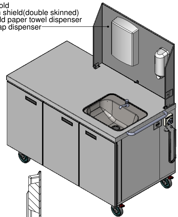
Isometric View
