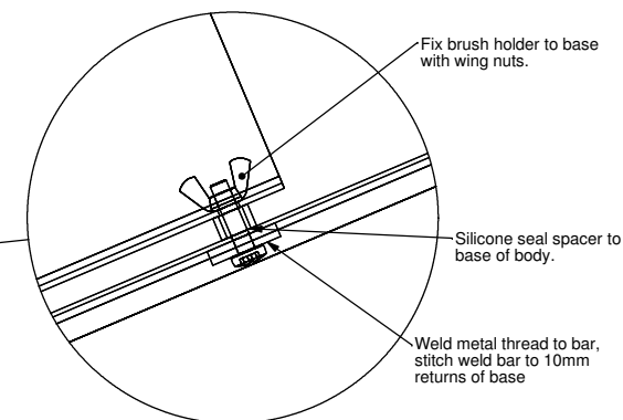
DETAIL T SCALE 1 : 2
