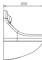
End View
